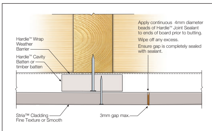
FIGURE 27 OFF-STUD JOINT
