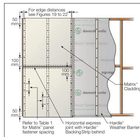
FIGURE 15 MATRIX™ PANEL FASTENERS
