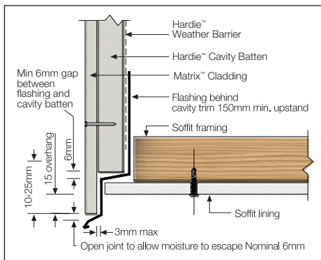
FIGURE 33 FACADE/SOFFT JUNCTION
