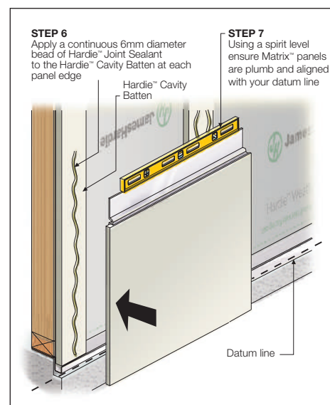
FIGURE 14 INSTALL FIRST PANEL
