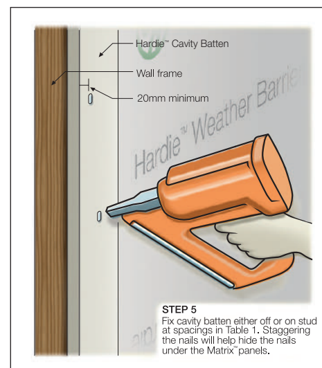
FIGURE 8 FIXING CAVITY BATTEN
