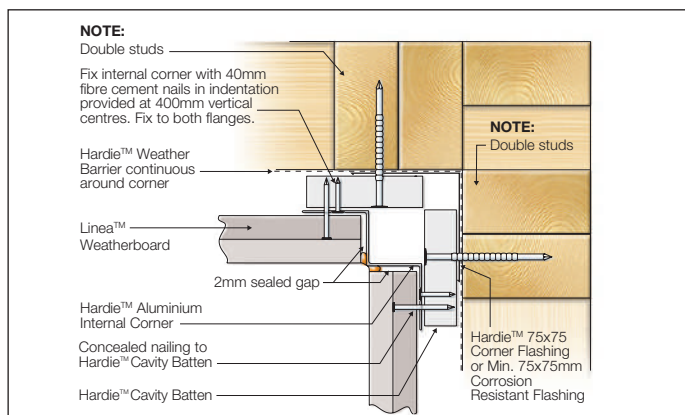
FIGURE 12 INTERNAL CORNER MOULD DETAIL
