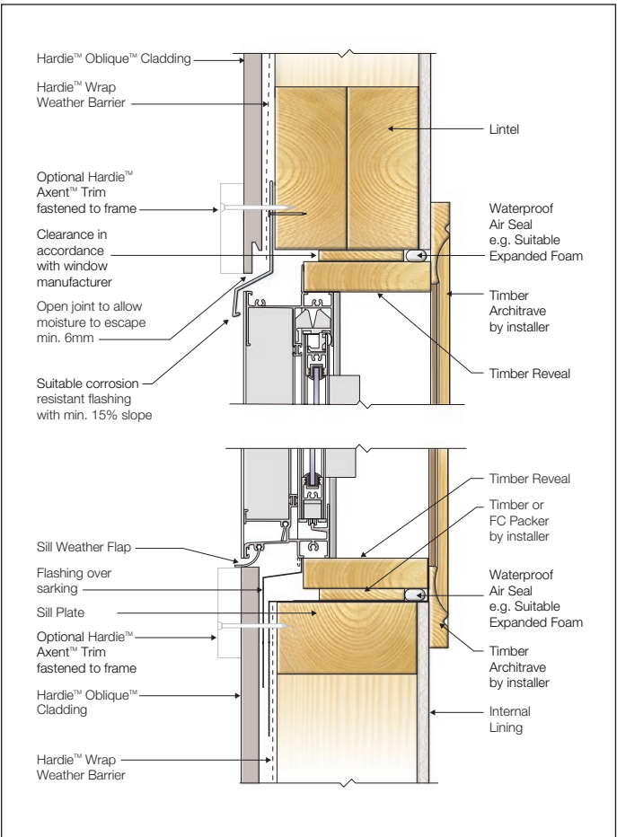
FIGURE 15 WINDOW HEAD AND SILL - TRIM
