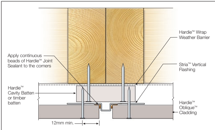
FIGURE 26 VERTICAL JOINT USING STRIA™ VERTICAL FLASHING STOP
