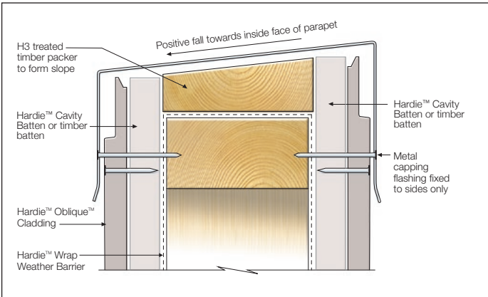
FIGURE 27 PARAPET DETAIL
