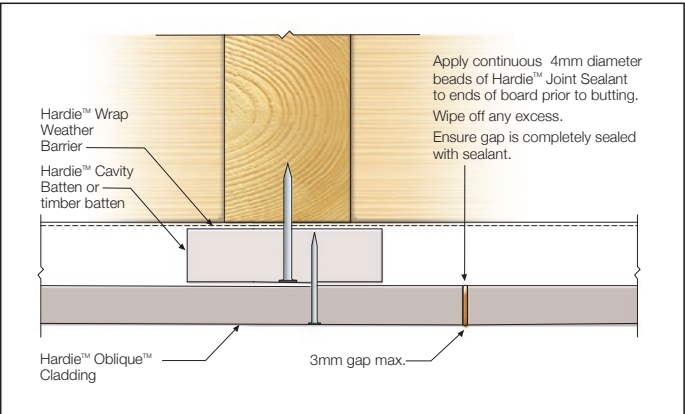
FIGURE 25 OFF-STUD JOINT
