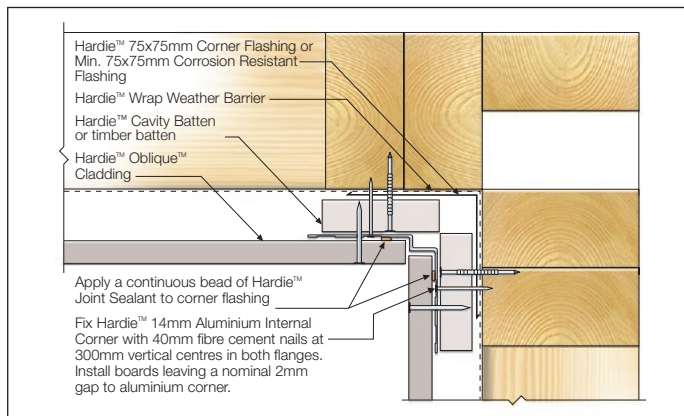
FIGURE 20 INTERNAL CORNER
