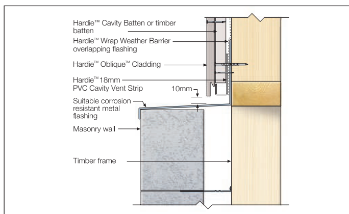
FIGURE 18 HORIZONTAL JUNCTION
