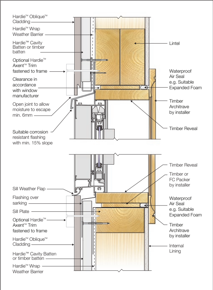
FIGURE 29 WINDOW HEAD AND SILL - TRIM
