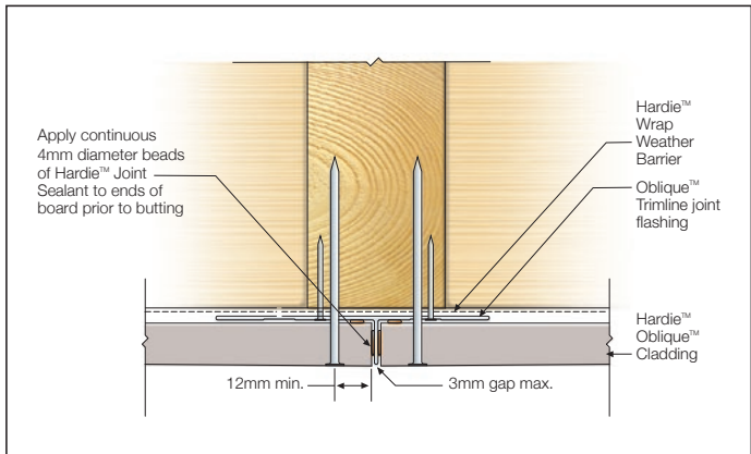
FIGURE 9 VERTICAL JOINT DETAIL
