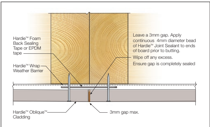
FIGURE 12 HARDIE™ FOAM BACK SEALING TAPE DETAIL
