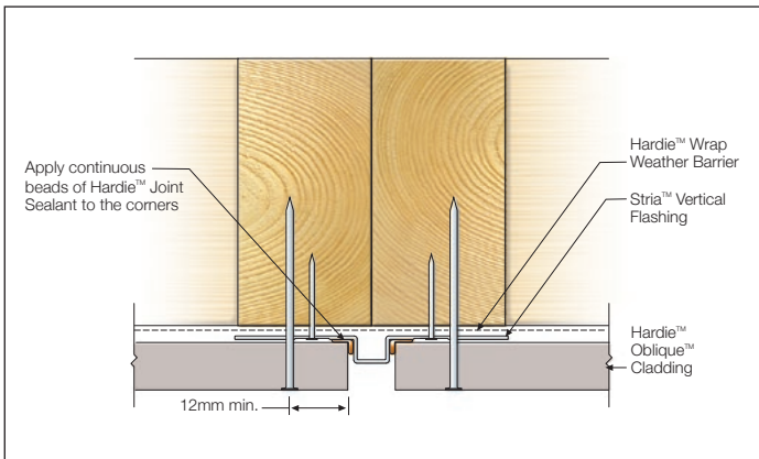
FIGURE 11 VERTICAL JOINT USING STRIA™ VERTICAL FLASHING STOP
