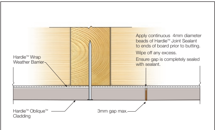
FIGURE 10 OFF-STUD JOINT
