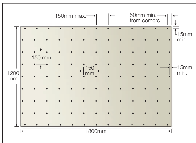
FASTENER NAILING PATTERN
