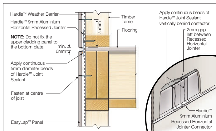
FIGURE 5 UPPER FLOOR JUNCTION OPTION 1
