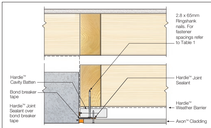
FIGURE 19 ABUTMENT DETAIL
