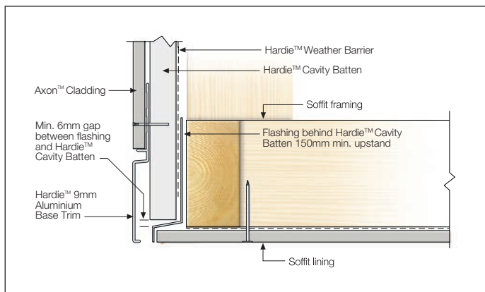
FIGURE 21 FACADE/SOFFIT JUNCTION
