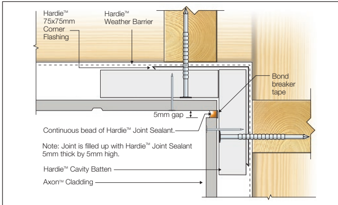
FIGURE 25 SEALANT FILL OPTION - CAVITY BATTEN
