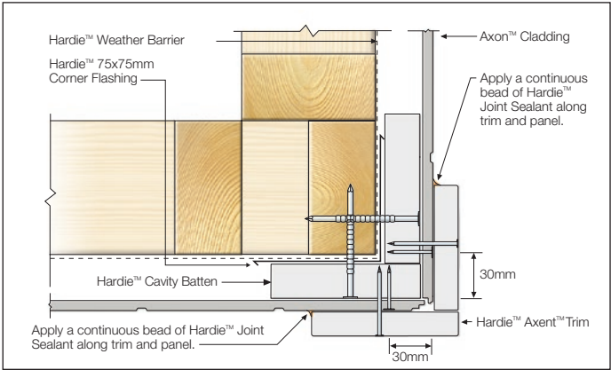
FIGURE 23 TRIM CORNER OPTION - CAVITY BATTEN
