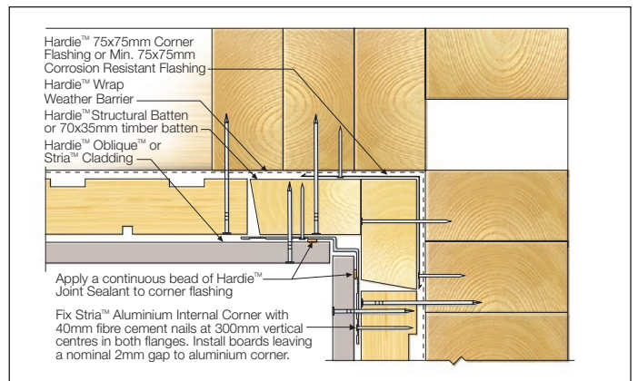
FIGURE 4 INTERNAL CORNER
