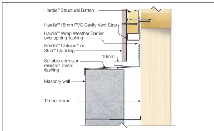
FIGURE 3 HORIZONTAL JUNCTION
