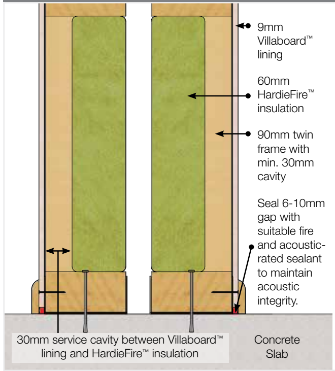
FIGURE 3 HARDIESMART™ INTERTENCY WALL SYSTEM BASE TO SLAB DETAIL
