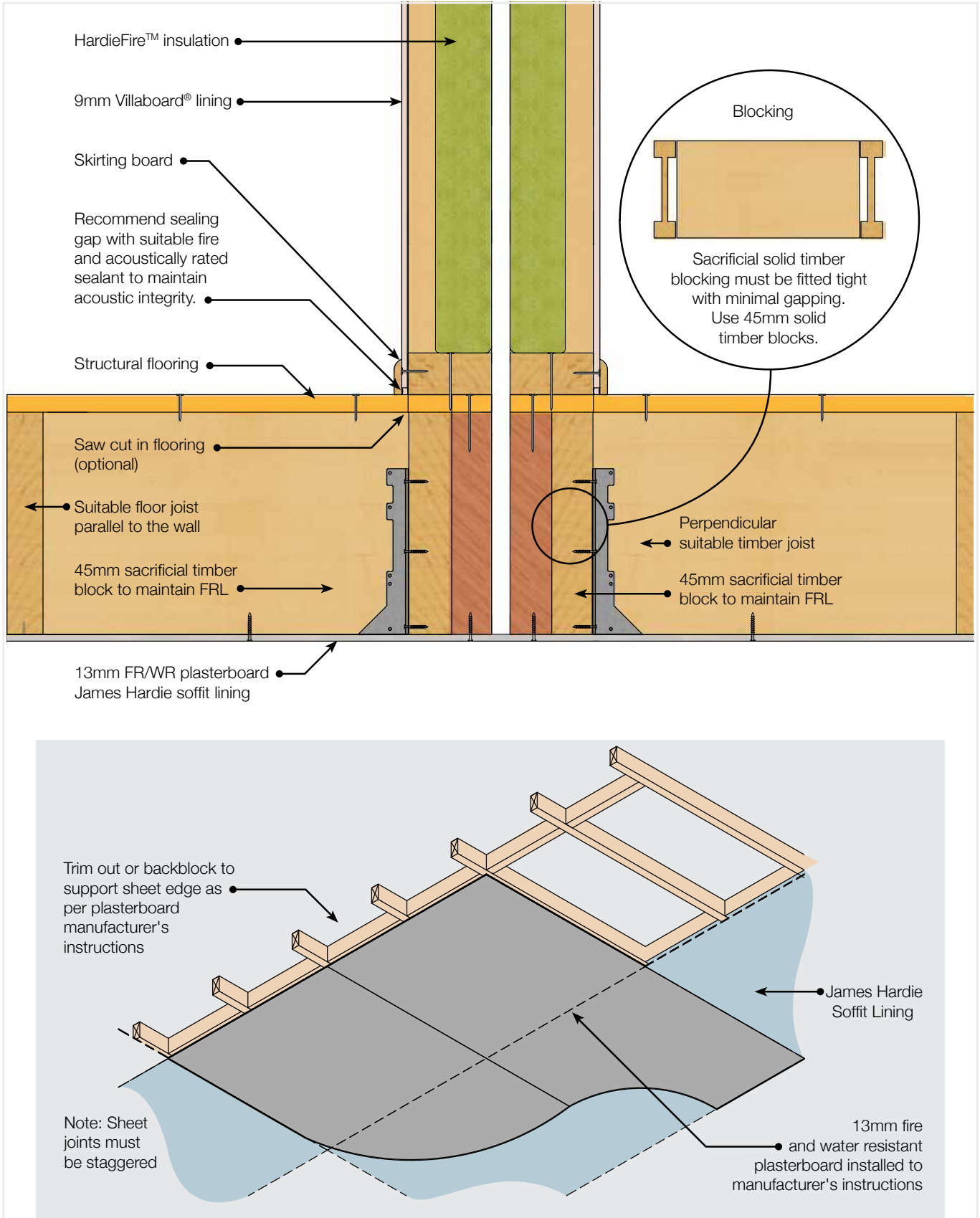
FIGURE 13 HARDIESMART™ INTERTENANCY WALL SYSTEM WITH CANTILEVERED FLOOR
