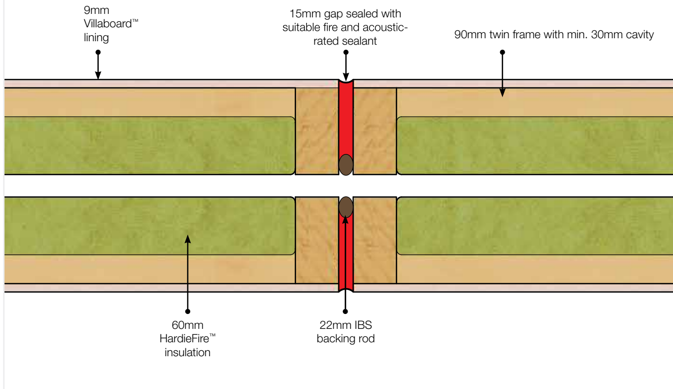
FIGURE 28 HARDIESMART™ INTERTENANCY WALL CONTROL JOINT
