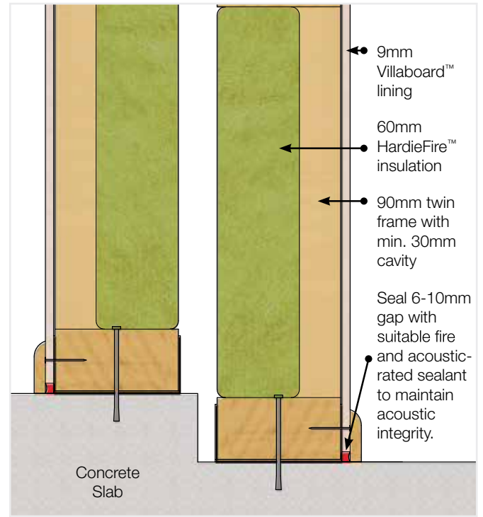
FIGURE 4 HARDIESMART™ INTERTENCY WALL SYSTEM BASE TO STEPPED SLAB DETAIL
