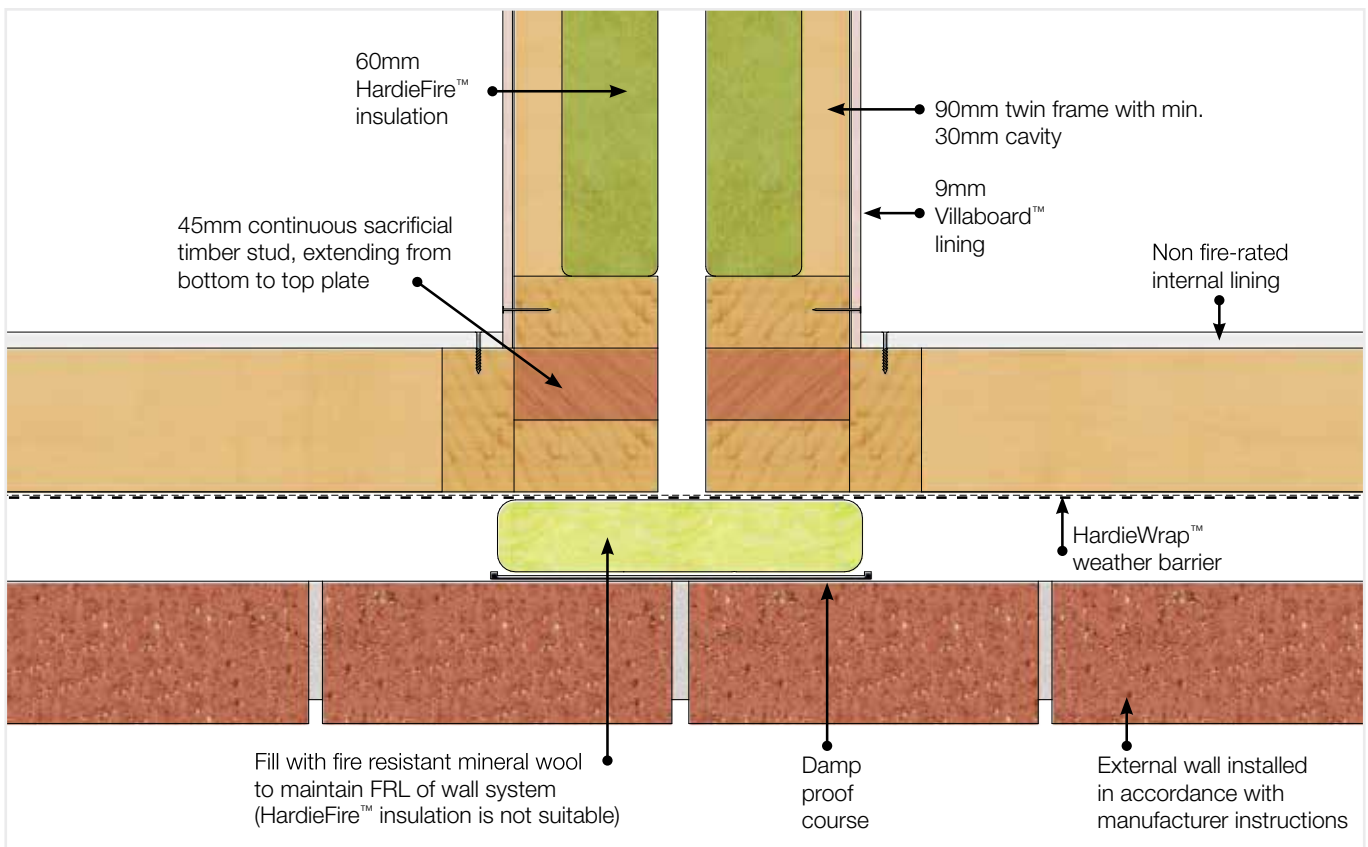
FIGURE 27 HARDIESMART™ INTERTENANCY WALL SYSTEM TO NON FIRE-RATED EXTERNAL CLADDING WALL
